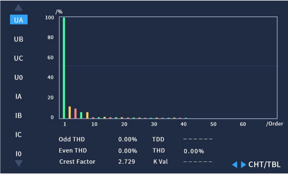
Fig. 4.15 Harmonics Chart
