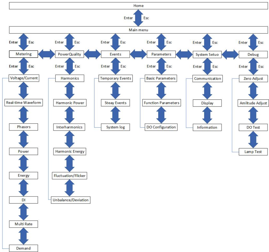
Fig. 4.2 Quick navigation
