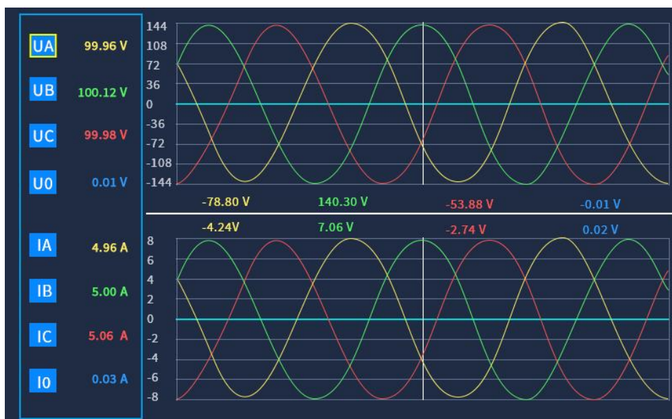
Fig. 4.7 Real-time Waveform
