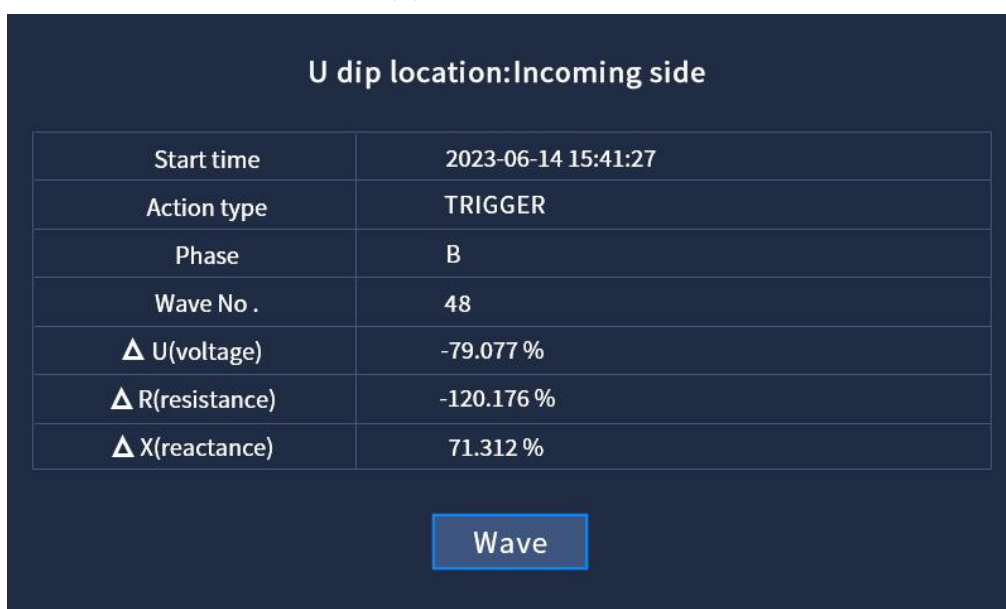
Fig. 4.27(a) Voltage dip location:incoming side
