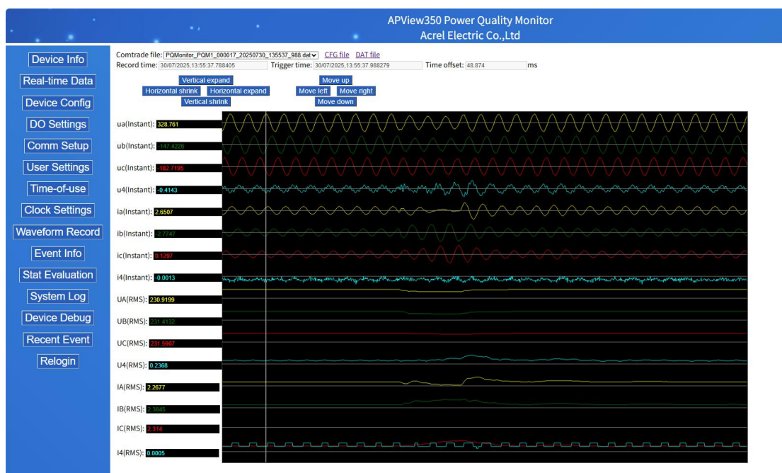
Fig. 1.5 Waveform Screen
