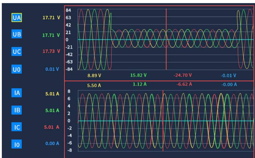
Fig. 4.24(b) Voltage dip waveform
