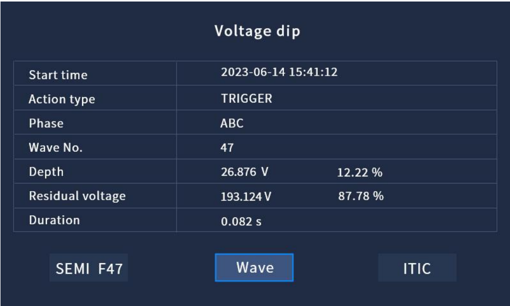
Fig. 4.24(a) Voltage dip
