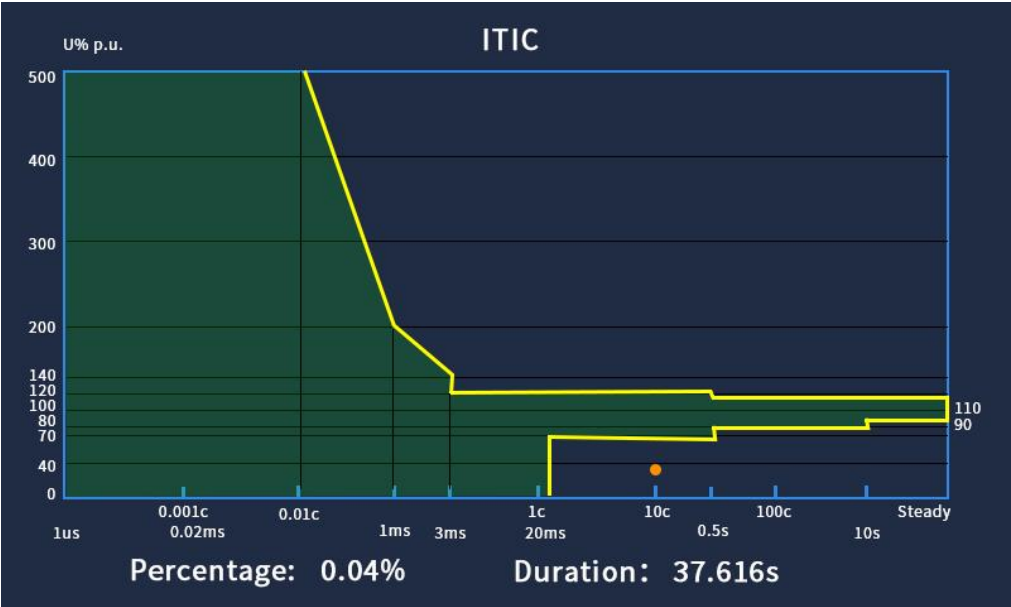
Fig. 4.28(a) ITIC Curves
