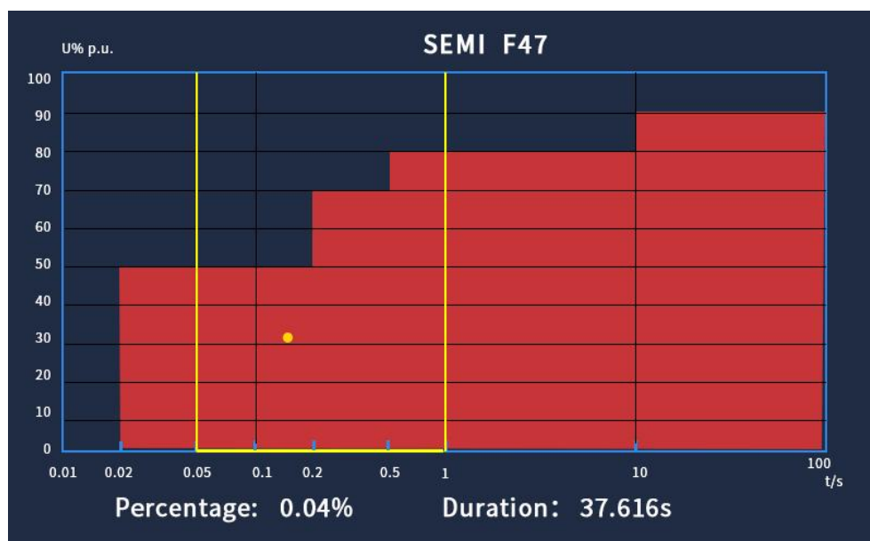
Fig. 4.28(b) SEMI F47 Curves
