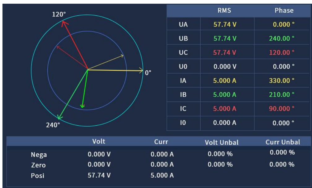
Fig. 4.8 Phasors
