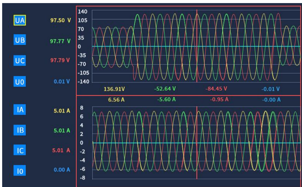
Fig. 4.25(b) Voltage swell waveform
