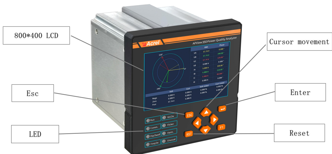
Fig. 4.1 Front Panel
