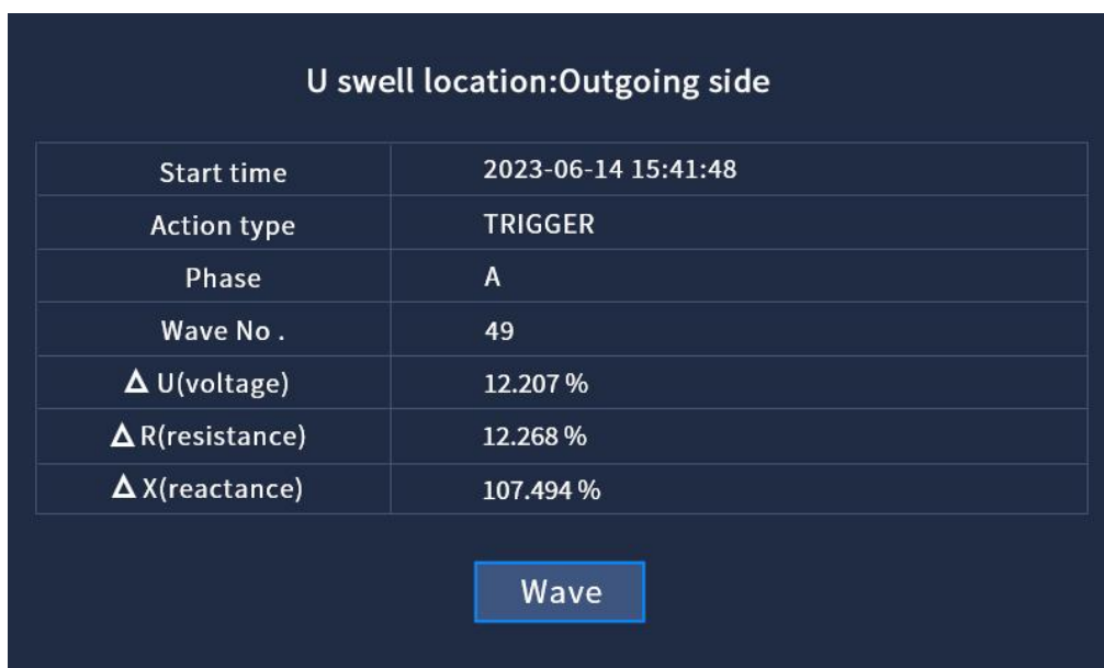
Fig. 4.27(b) Voltage swell location:Outgoing side
