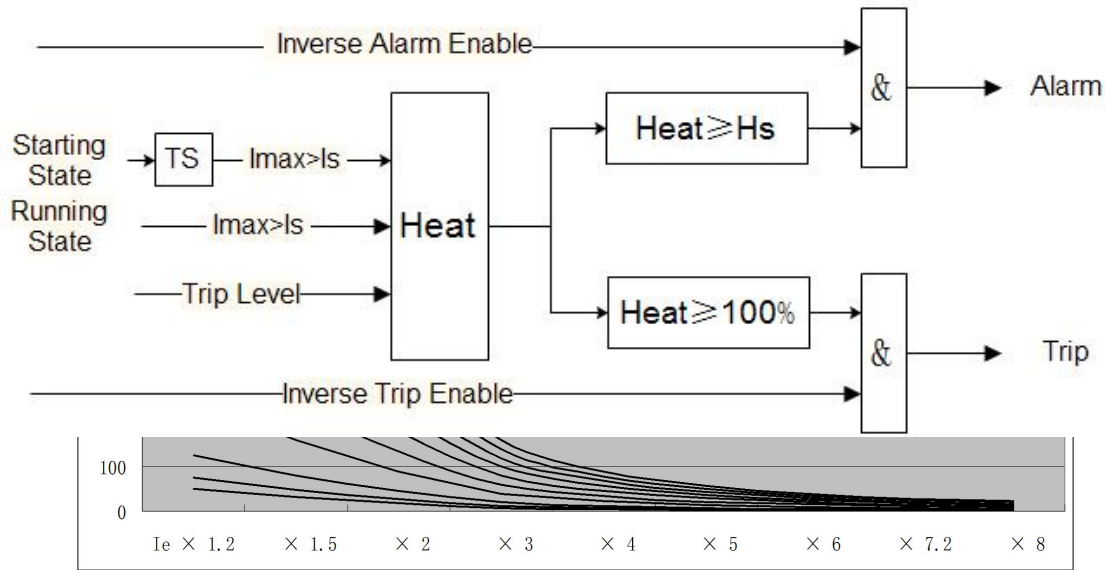
Figure 10 Characteristic curve of overload (K curve)
