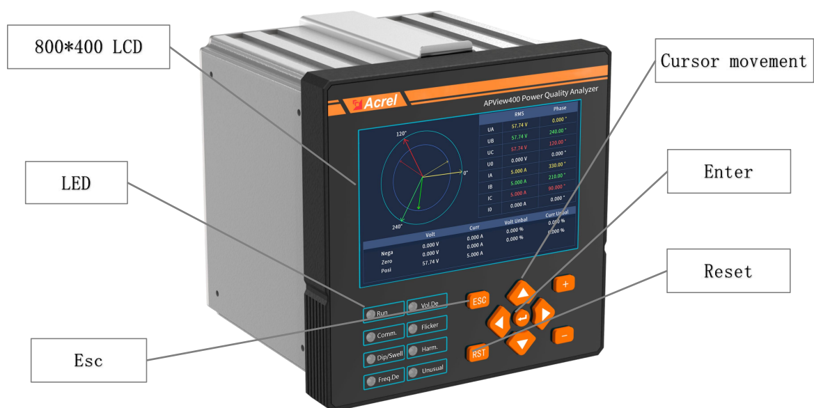
Fig. 4.1 Front Panel
