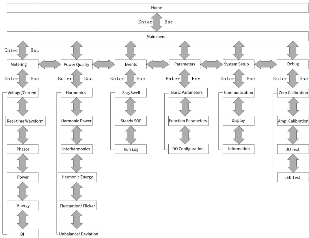
Fig. 4.2 Quick navigation
