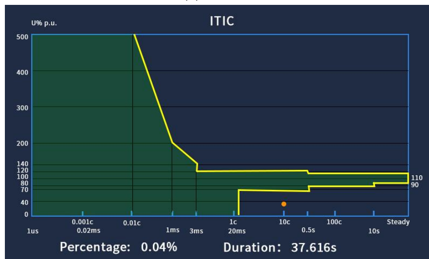
Fig. 4.26(a) ITIC Curves
