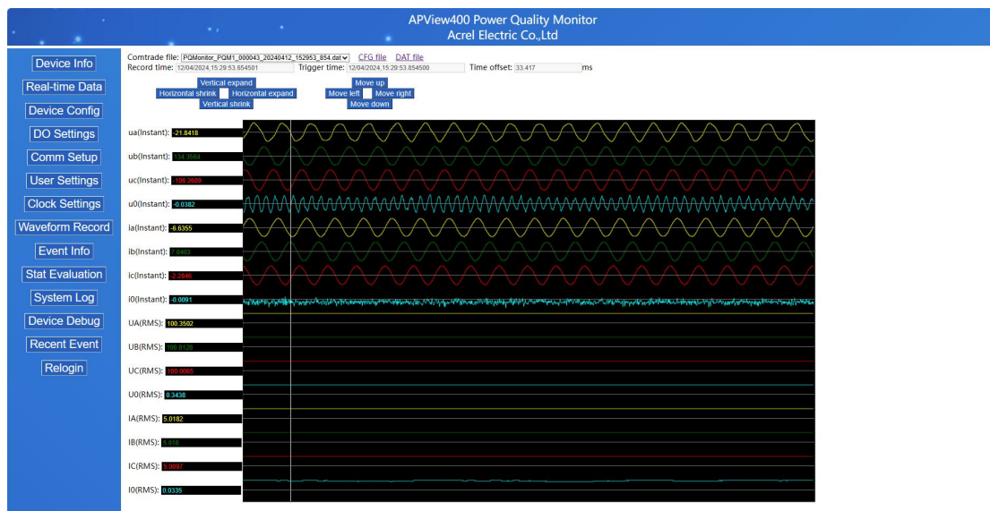
Fig. 1.5 Waveform Screen
