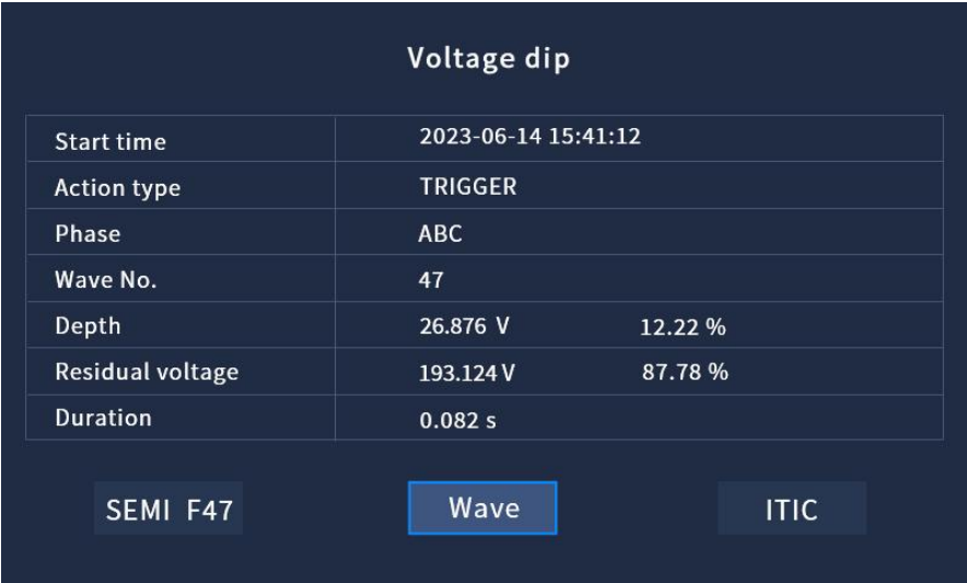
Fig. 4.22(a) Voltage dip
