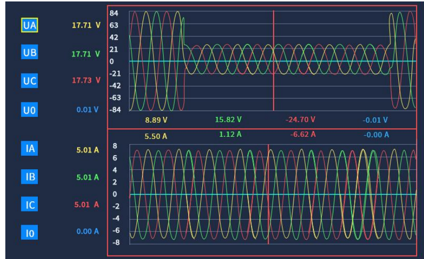
Fig. 4.22(b) Voltage dip waveform
