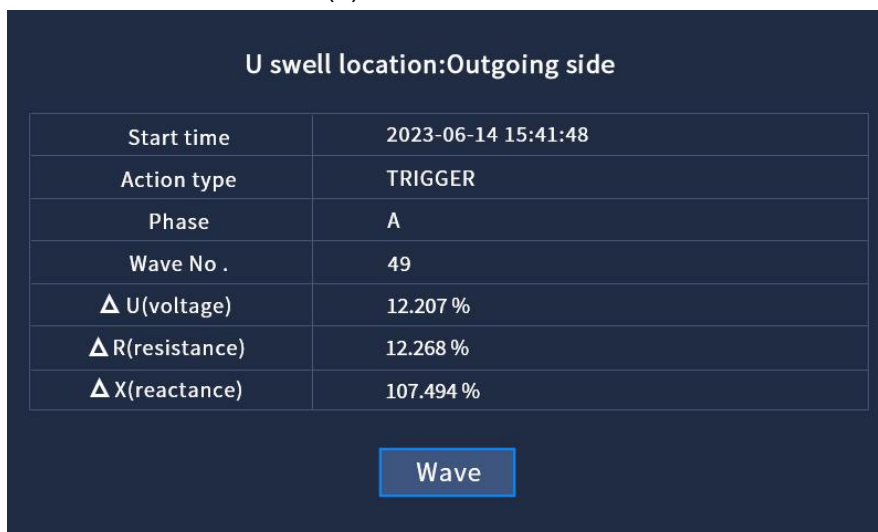
Fig. 4.25(b) Voltage swell location:Outgoing side
