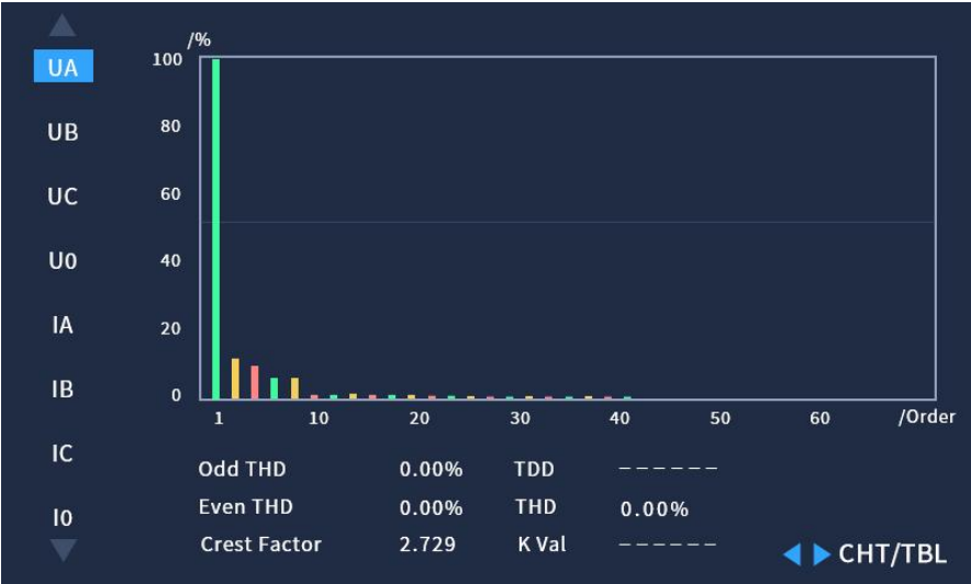
Fig. 4.13 Harmonics Chart
